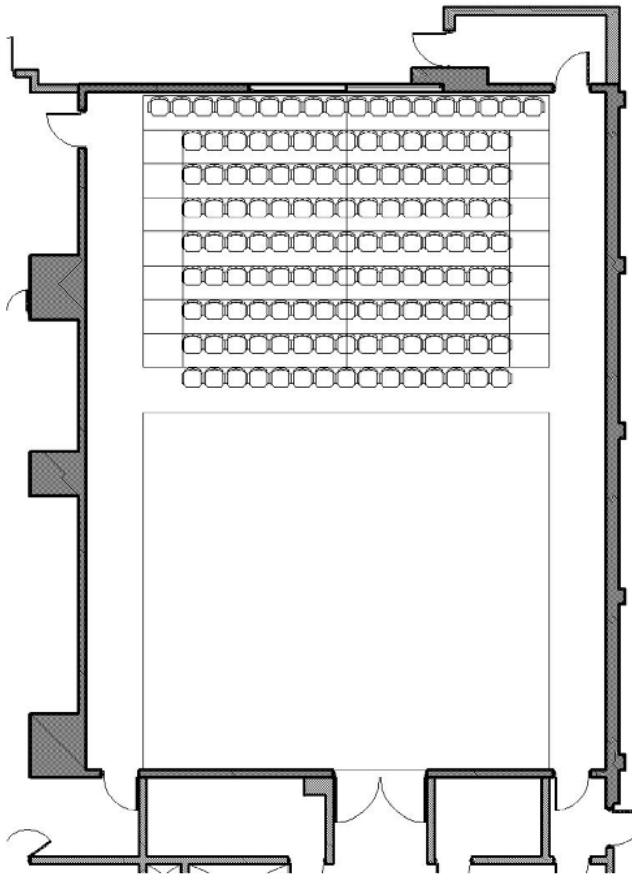
36' x 31'-8" Stage
